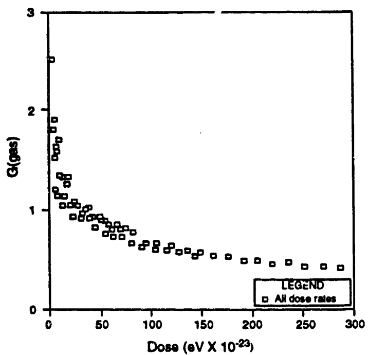
Fig. 2. Decrease in G(gas) with increasing dose. For cellulose.
